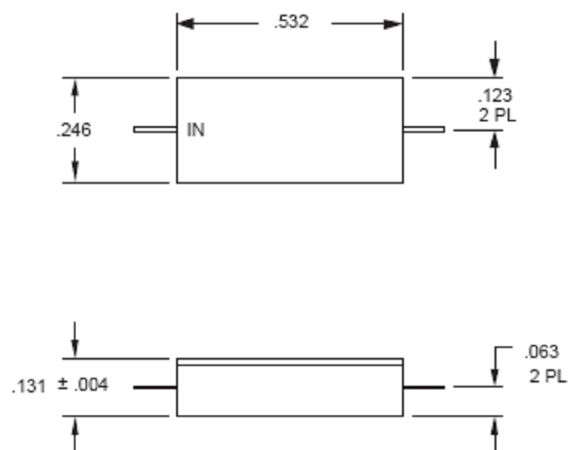
210019 OUTLINE
