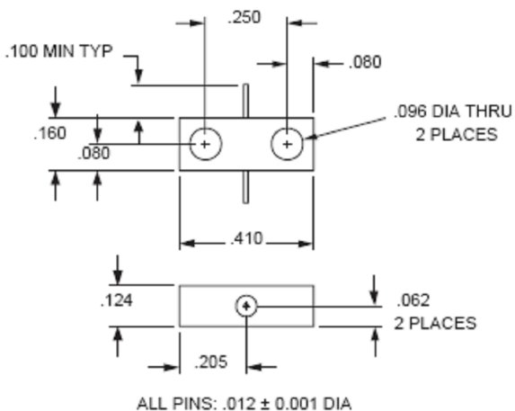
210032 OUTLINE
