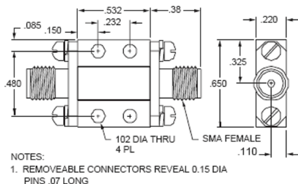
210032 OUTLINE
