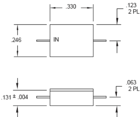
210013 OUTLINE
