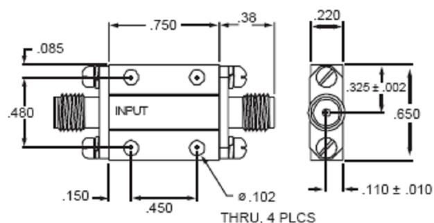
210093 OUTLINE
