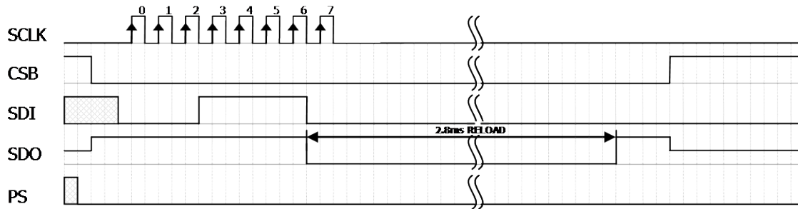
Figure 4: Reset command sequence SPI mode 0
