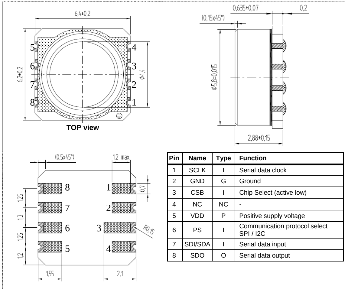
Figure 17: MS5803-01BA07 package outlines, pin configuration and description
