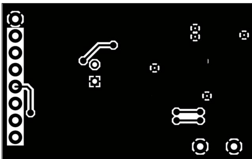
Figure 2-4. Atmel ATA6620/23/25 Development Board; Bottom Side, Top View (as if PCB Were Transparent)
