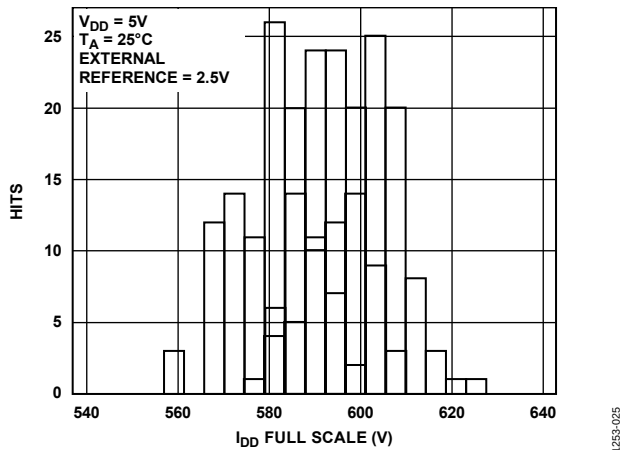
Figure 23. I_{DD} Histogram with External Reference
