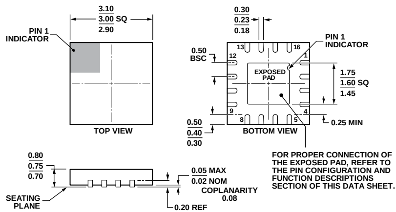
Figure 52. 16-Lead Lead Frame Chip Scale Package [LFCSP_WQ] 3 mm × 3 mm Body, Very Very Thin Quad (CP-16-22)
