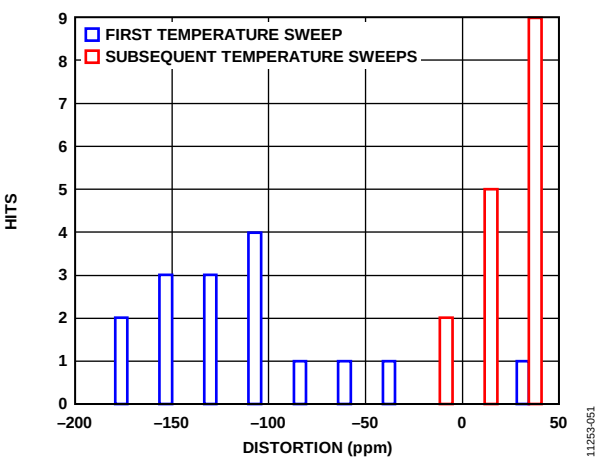
Figure 48. Thermal Hysteresis
