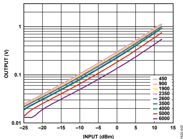
Figure 7. PEAK Output vs. Input Level, 450 MHz, 900 MHz, 1900 MHz, 2350 MHz, 2600 MHz, 3500 MHz, 4000 MHz, 5000 MHz, 6000 MHz, Supply 3.0 V
