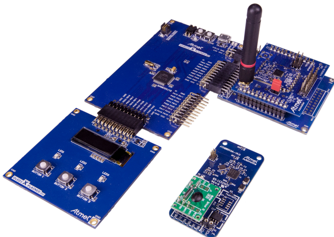
Figure 1-2. ATA8510-EK1 Kit
