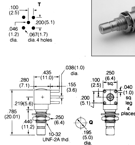
SMB PCB Angle Bulkhead Receptacle Male Contact/Four Legs/No Stand-off Pads 903-376J-51A Tin Lead Plated Cube Body & Legs, Gold Plated Interface & Contact
