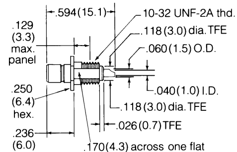
SMB Bulkhead Receptacle-Front Mount Male Contact/Solder Cup Terminal 903-406J-51R ▲ □ Gold Plated
