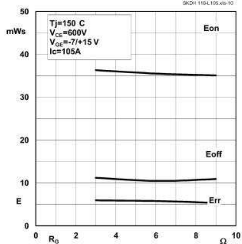
Fig. 10 turn-on/-off energy = f(R_g)
