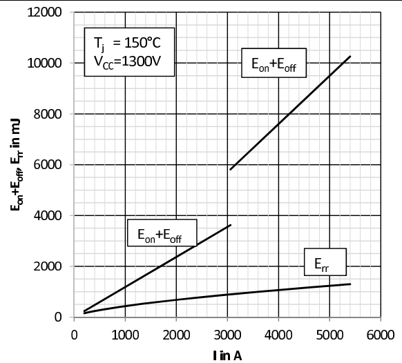
Fig. 4: Typical switching energy E = f(I_C)
