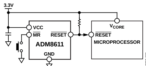
Figure 30. ADM8611 Typical Application Circuit
