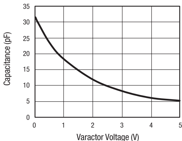
Figure 1. Capacitance vs Voltage ( T_J = 25^\circ C )
