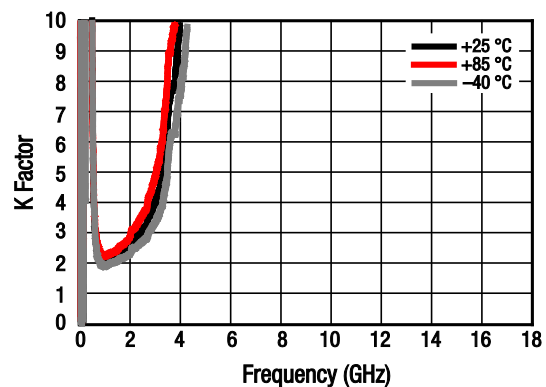
Figure 13. Stability Factor (K) vs Frequency Over Temperature
