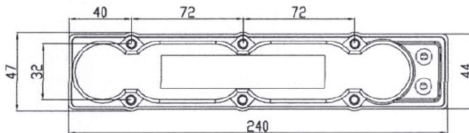
Prior mounting hole location dimensions
