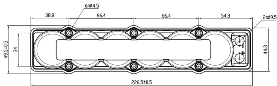
New mounting hole location dimensions
