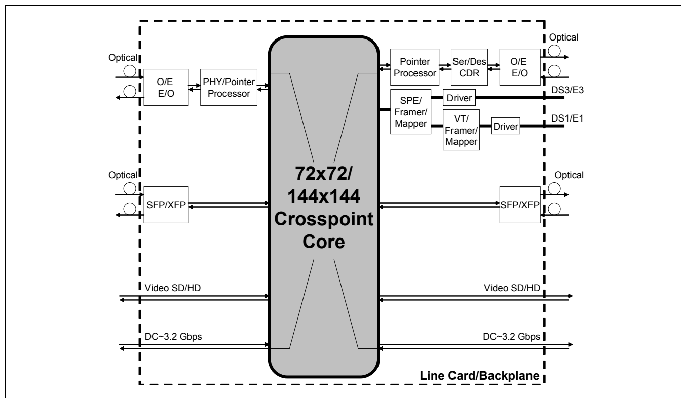
Figure 4-4. Crosspoint Application Example
