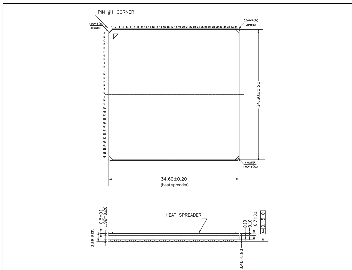
Figure 2-1. M21131/M21151 (-12/-13/-14) Package Outline Top View and Cross Sectional View (in mm)
