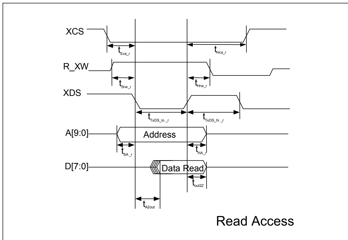
Figure 4-6. Parallel Read Timing Diagram
