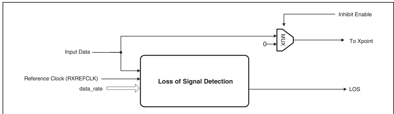
Figure 4-11. LOS Architecture
