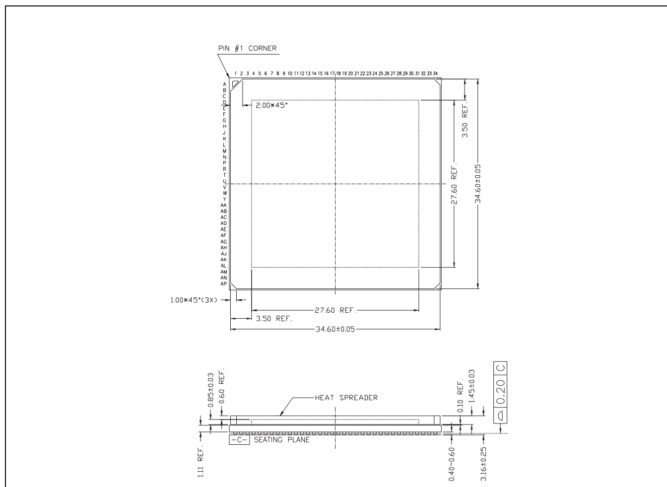
Figure 2-3. M21131/M21151 (-22/-23/-24) Package Outline Top View and Cross Sectional View (in mm)
