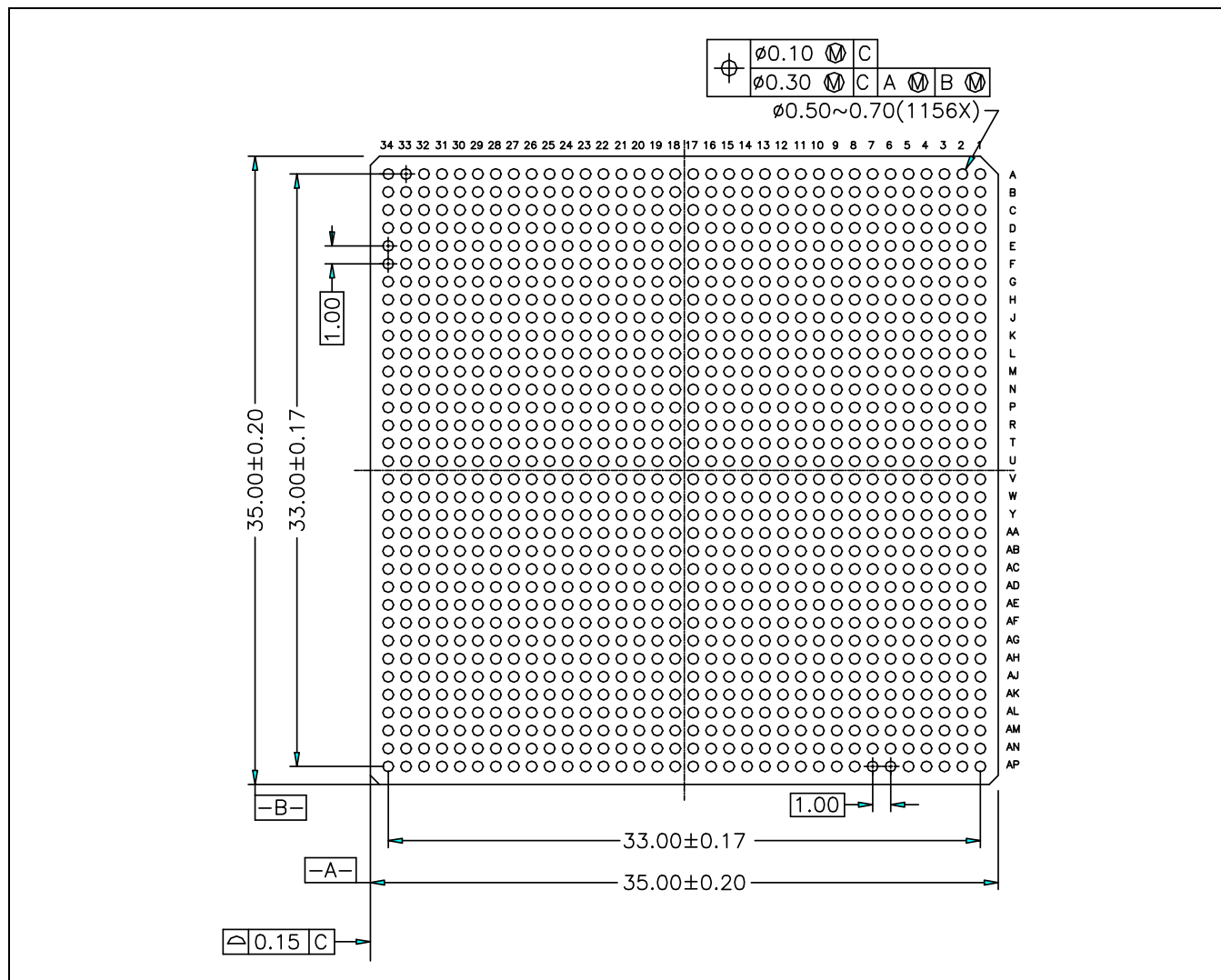
Figure 2-2. M21131/M21151 (-12/-13/-14) Bottom View of Package (in mm)
