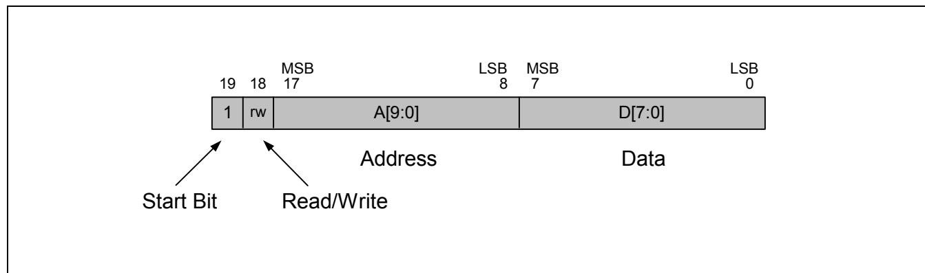
Figure 4-7. Serial Word Format
