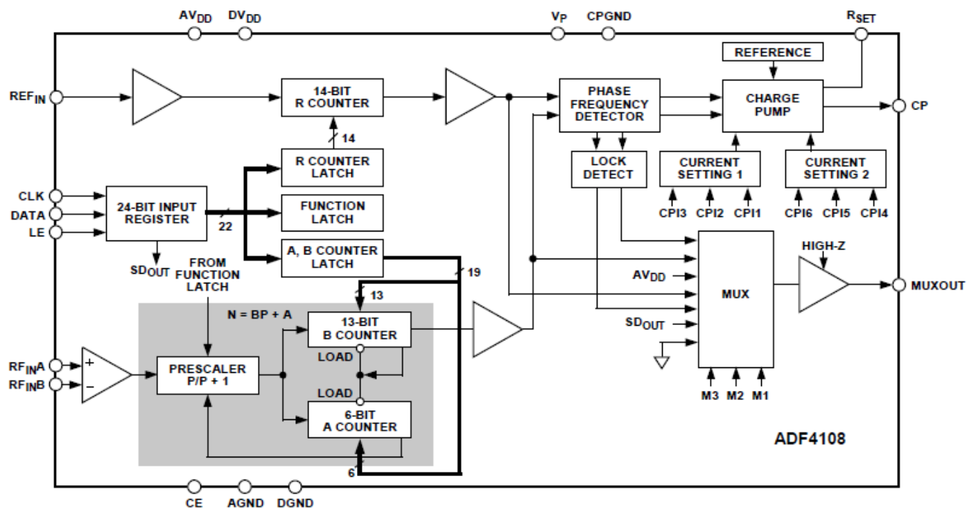
Figure 3 – Block Diagram.
