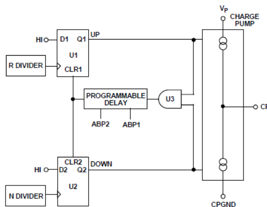
Figure 7. PFD Simplified Schematic and Timing (in Lock)
