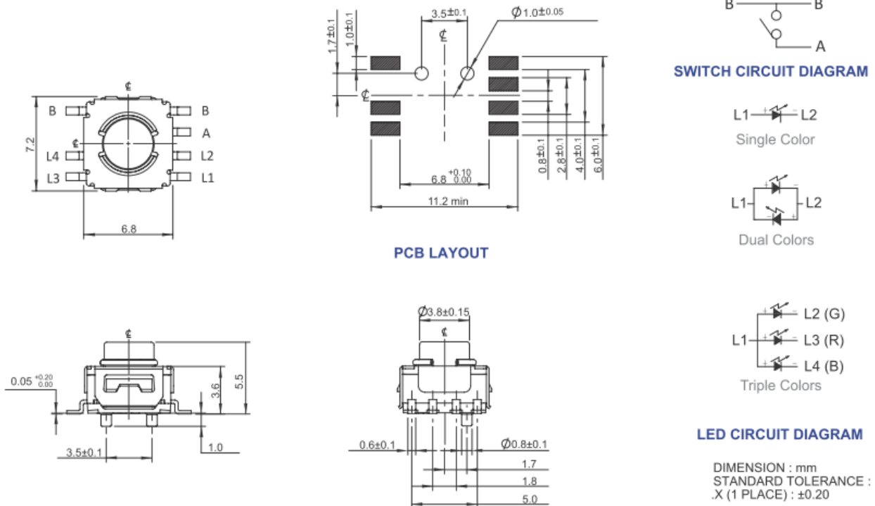
Figure 1 – 228EMV, Surface Mount Gull Wing, Vertical Actuation
