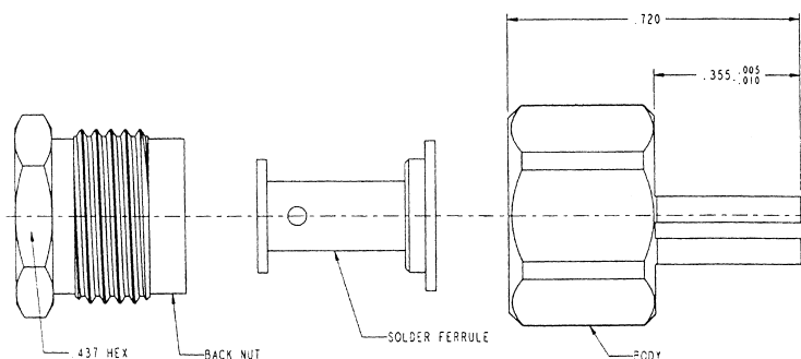
716-101 Edge Board Mount for 0.141 S/R Cable
