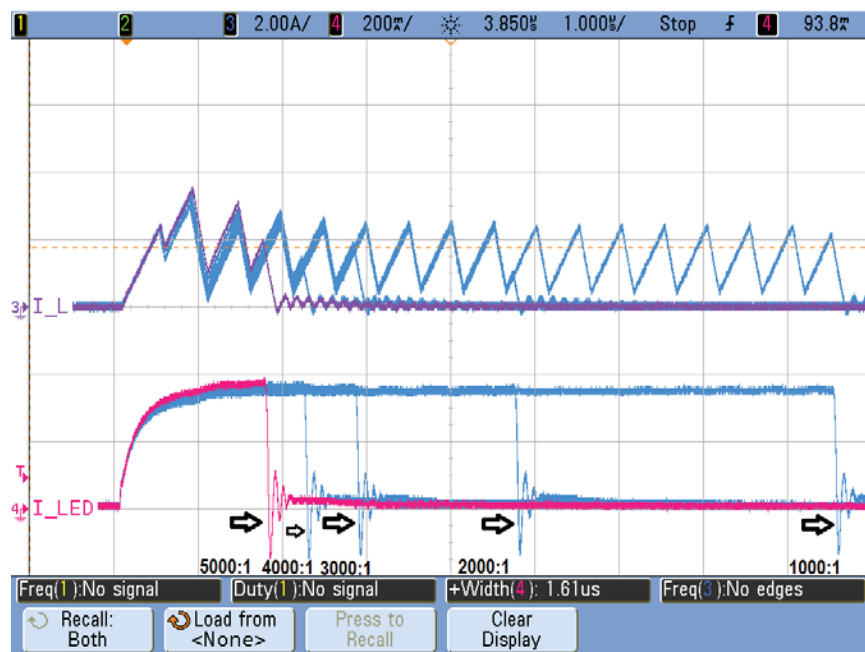
Figure 2. DC2361A 12V IN 120Hz PWM Dimming Waveforms at Different PWM Duty Cycles with 5000:1 in Bold. I LED Waveform (200mA/Div) Is on the Bottom (with 40V LED String) and I L Waveform (2A/Div) Is on the Top.
