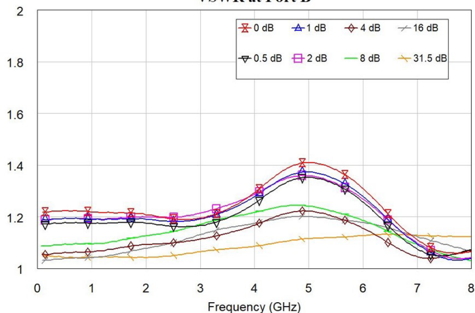
VSWR at Port B
