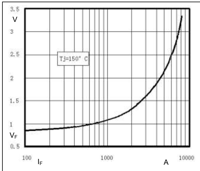
Fig1. Forward Characteristics
