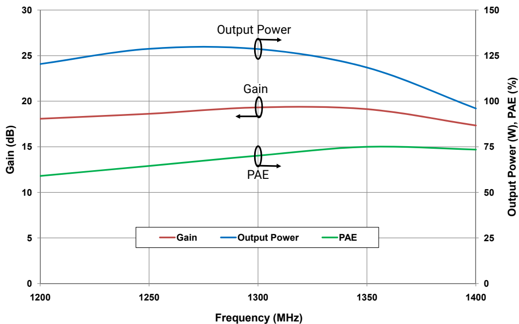
Gain, Output Power and PAE vs Frequency measured in Broadband Amplifier Circuit CGH40120F-AMP
