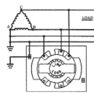
Fig. 6 Three Delta/One Phase Grounded
