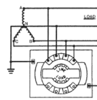
Fig. 4 Three Phase Wye/4 or 5 Wire/GND Neutral
