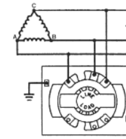
Fig. 5 Three Phase Delta/Ungrounded
