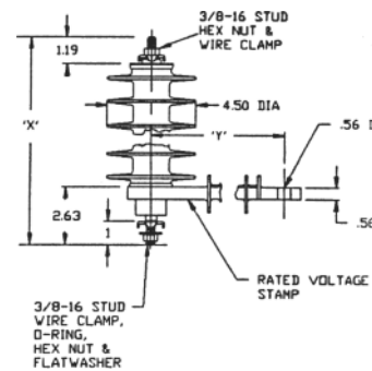
Tranquell™ distribution arrester, rated 10 kV, with disconnecter)
