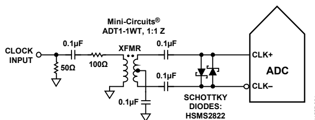
Figure 42. Transformer Coupled Differential Clock (Up to 200 MHz)
