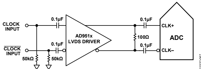
Figure 45. Differential LVDS Sample Clock (Up to 1 GHz)
