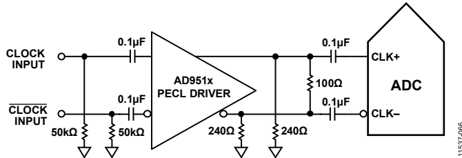
Figure 44. Differential PECL Sample Clock (Up to 1 GHz)
