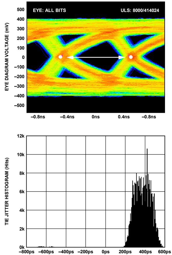
Figure 52. Data Eye for LVDS Outputs in ANSI-644 Mode with Trace Lengths of Greater Than 24 Inches on Standard FR-4 Material, External 100 \Omega Far End Termination Only
