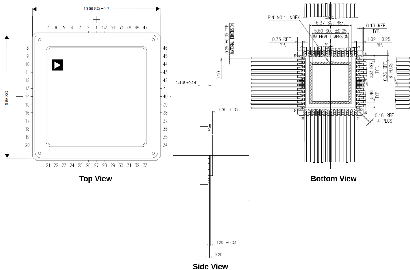
Figure 52-Lead Quad Flat Pack [CQCC] 10 mm × 10 mm Body 1
