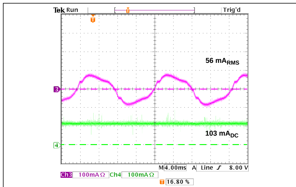
FIGURE D-5: AC Input Voltage at 270 \text{ V}_{\text{AC}} .
