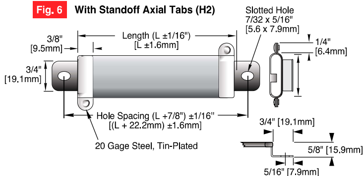
Fig. 6 With Standoff Axial Tabs (H2)
