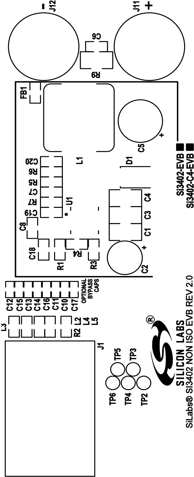
Figure 2. Top Silkscreen
