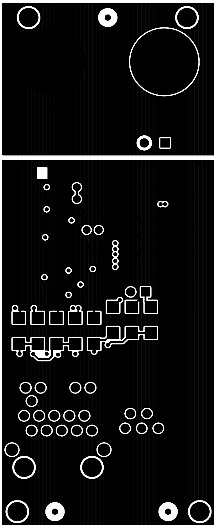
Figure 6. Bottom Layer
