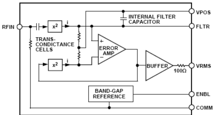
FIGURE 2. Block diagram.
