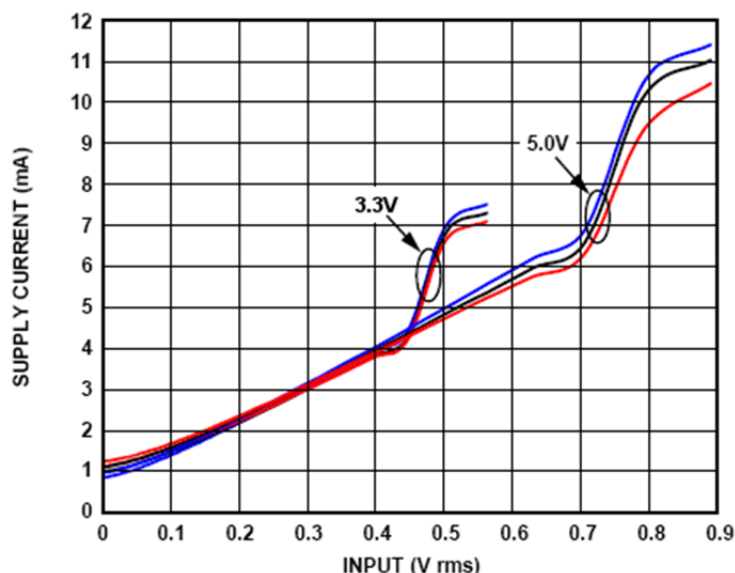
Figure 4. Supply current vs. input level; supplies = 3.3 V and 5.0 V; T_A = -55^\circ\text{C} , +25^\circ\text{C} , and +125^\circ\text{C} .
