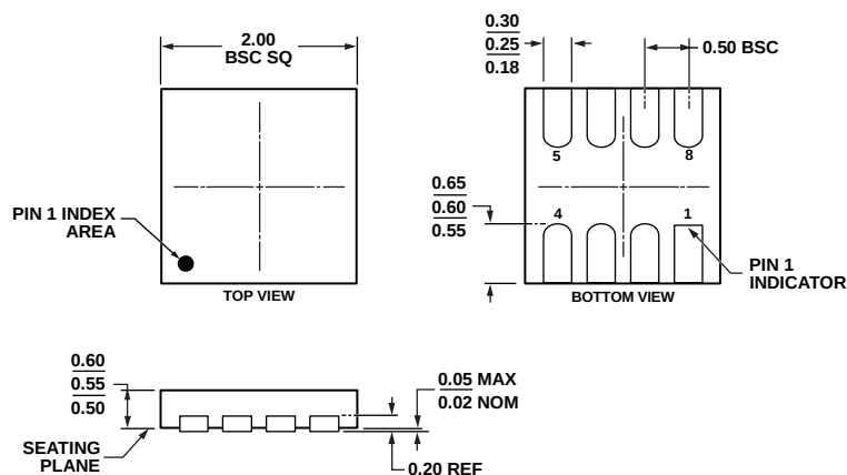
Figure 72. 8-Lead Lead Frame Chip Scale Package [LFCSF_WD] 2 mm x 2 mm Body, Very Very Thin, Dual Lead (CP-8-6)
