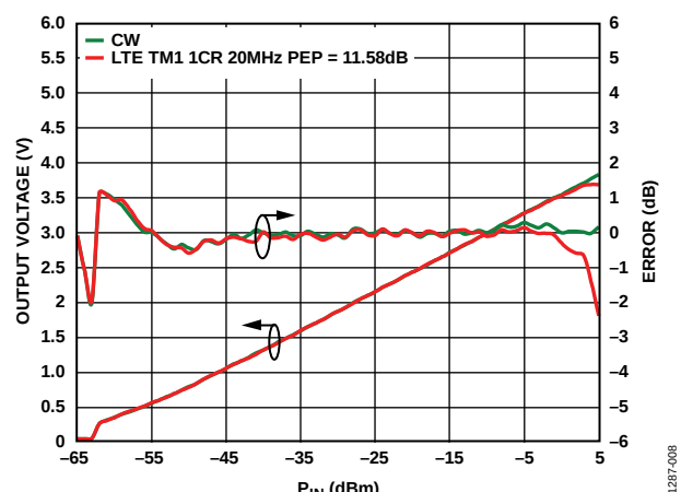
Figure 8. Error from CW Linear Reference vs. Signal Modulation (LTE TM1 One-Carrier, 20 MHz), Frequency = 2.14 GHz, C_{RMS} = 0.1 \mu F, Three Point Calibration at 0 dBm, -40 dBm, and -55 dBm
