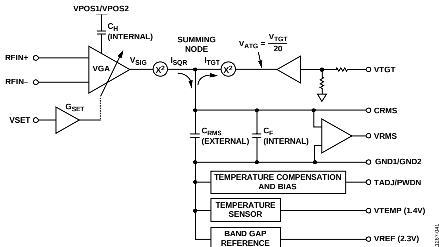
Figure 41. Simplified Architecture Details
