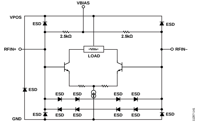
Figure 42. RF Inputs
