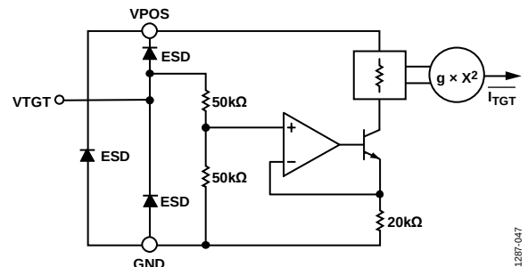
Figure 49. VTGT Interface
