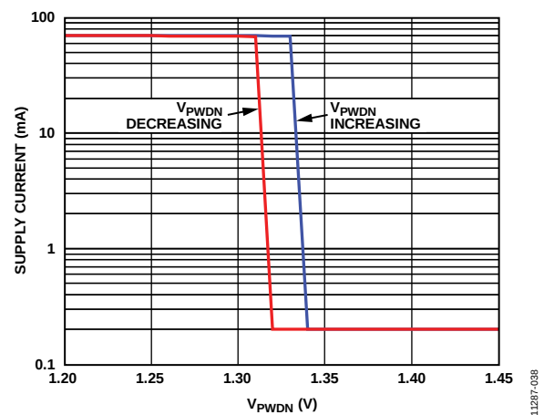
Figure 38. Supply Current vs. V_{PDN}
