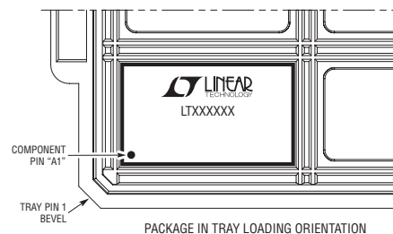
PACKAGE IN TRAY LOADING ORIENTATION
