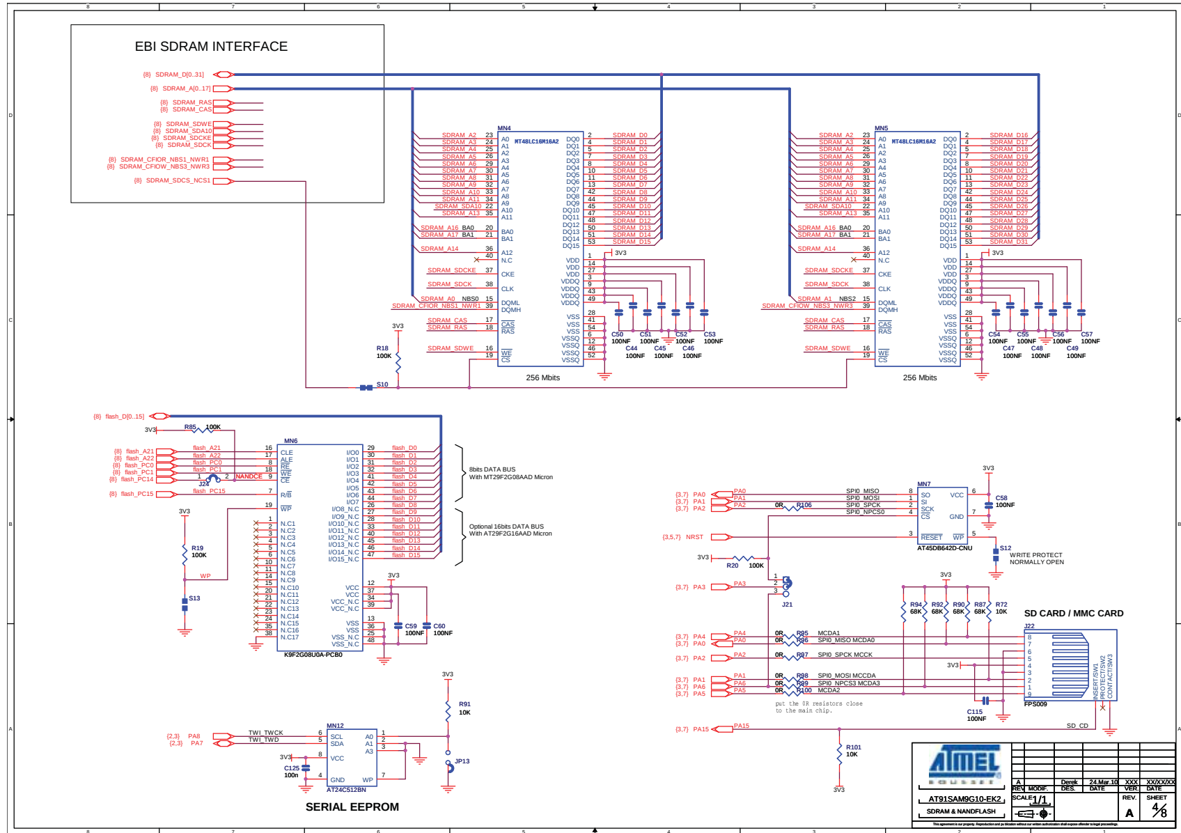
Figure 7-4. SDRAM and NAND Flash
