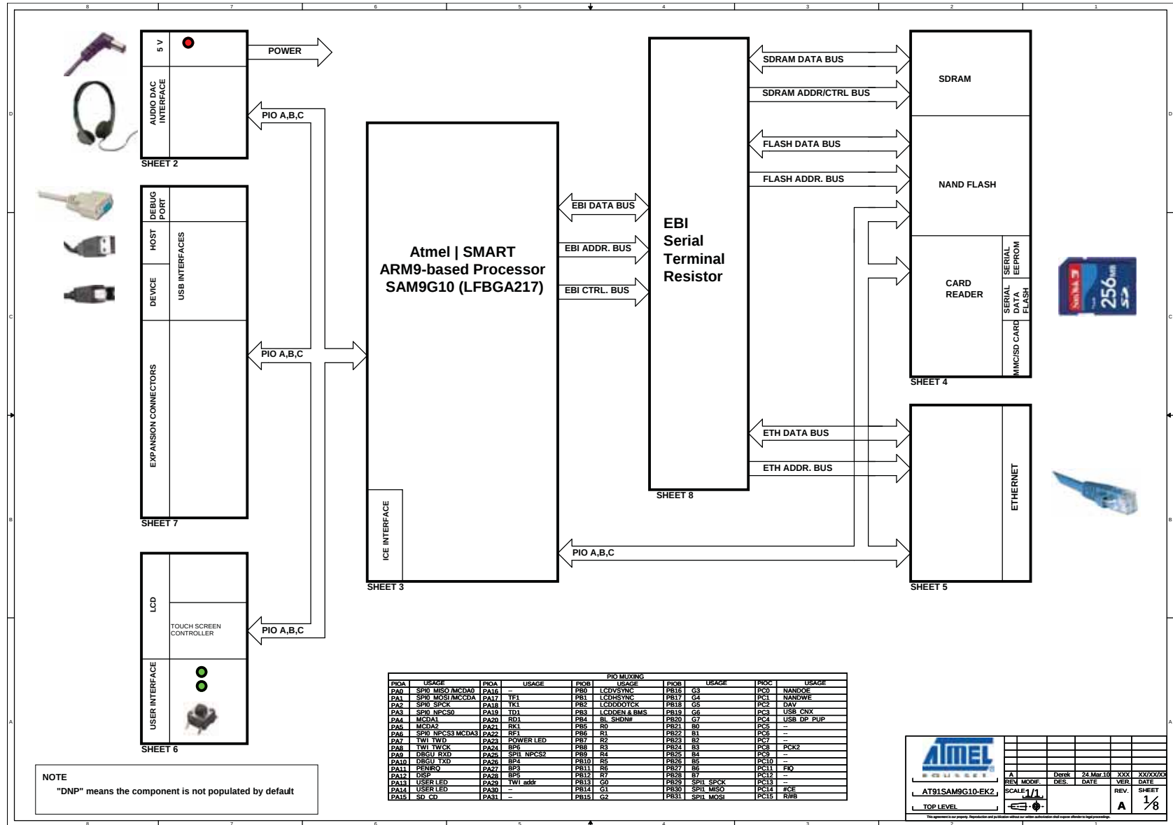
Figure 7-1. Board Architecture
