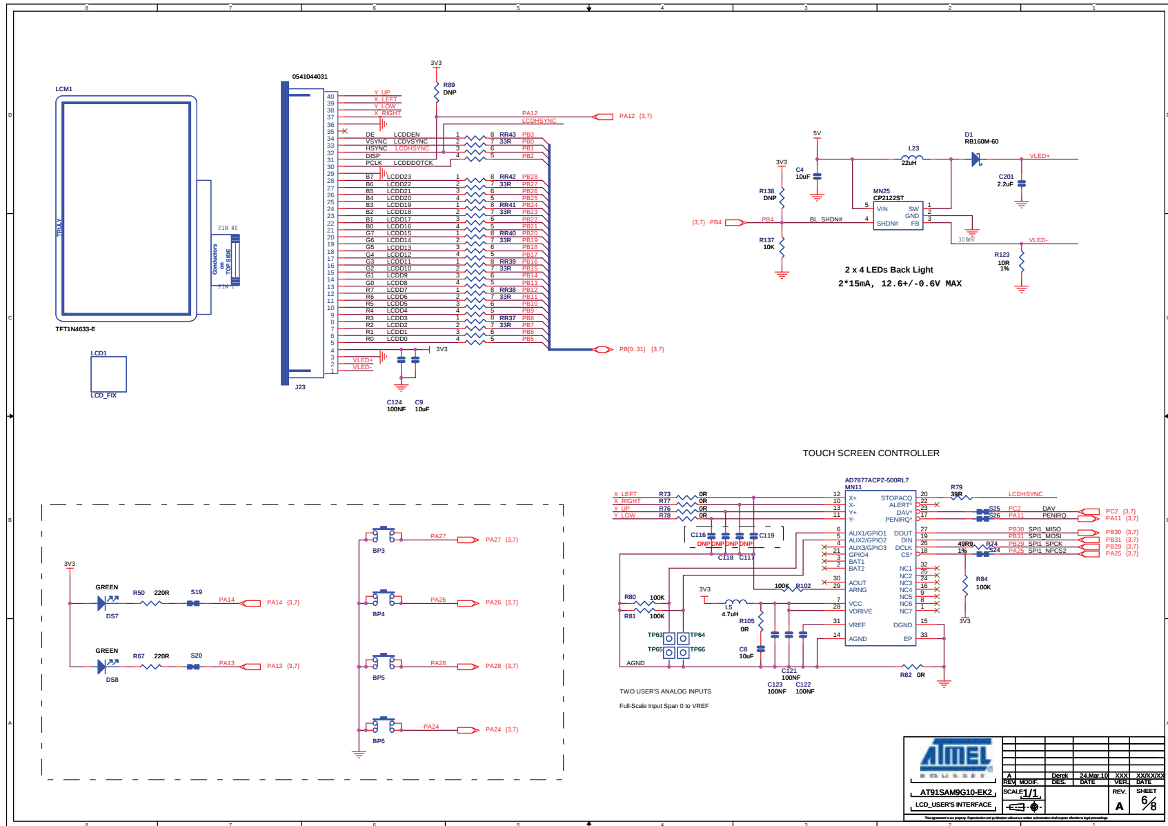
Figure 7-6. LCD and User Interface
