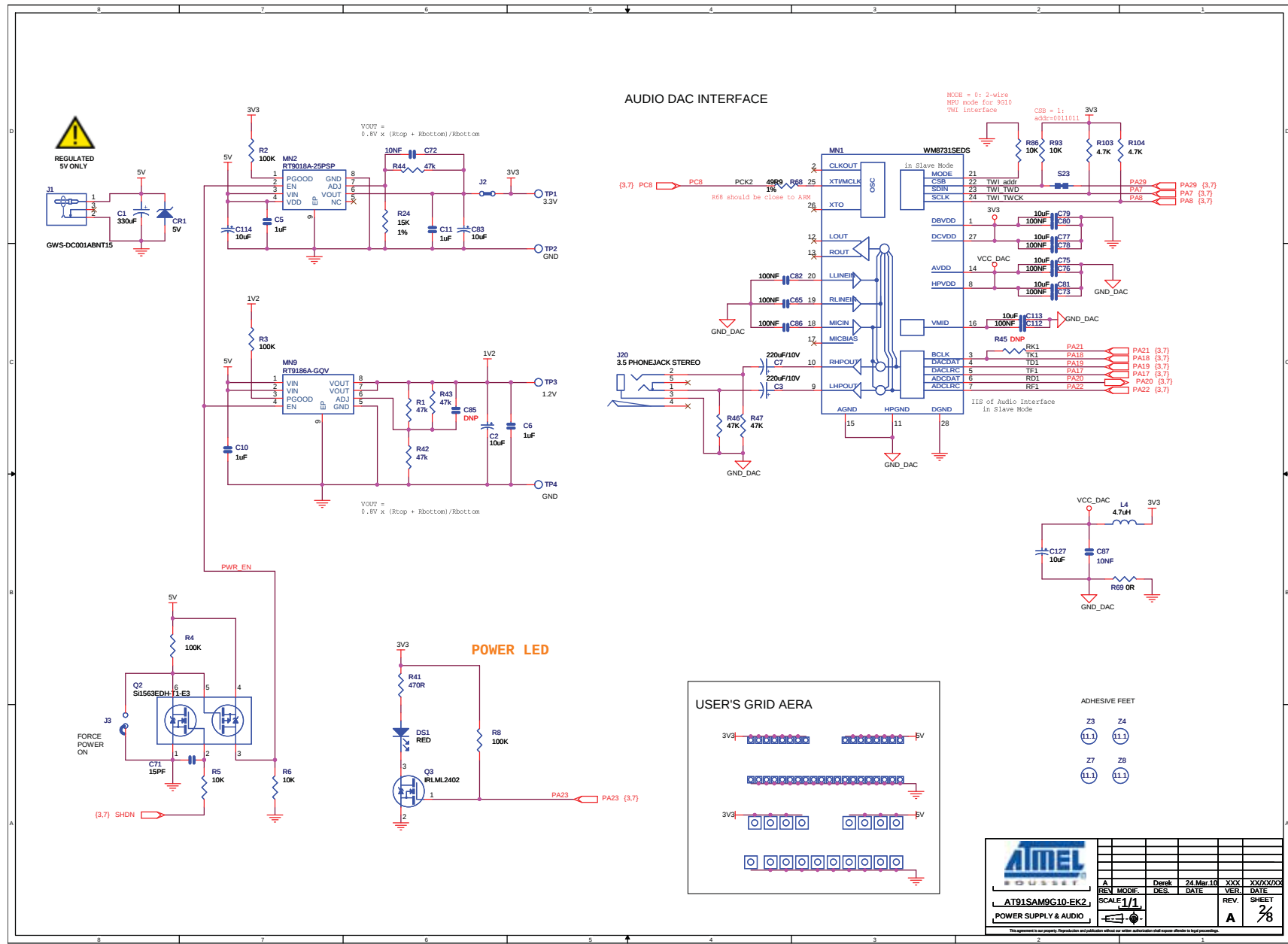
Figure 7-2. Power Supply and Audio
