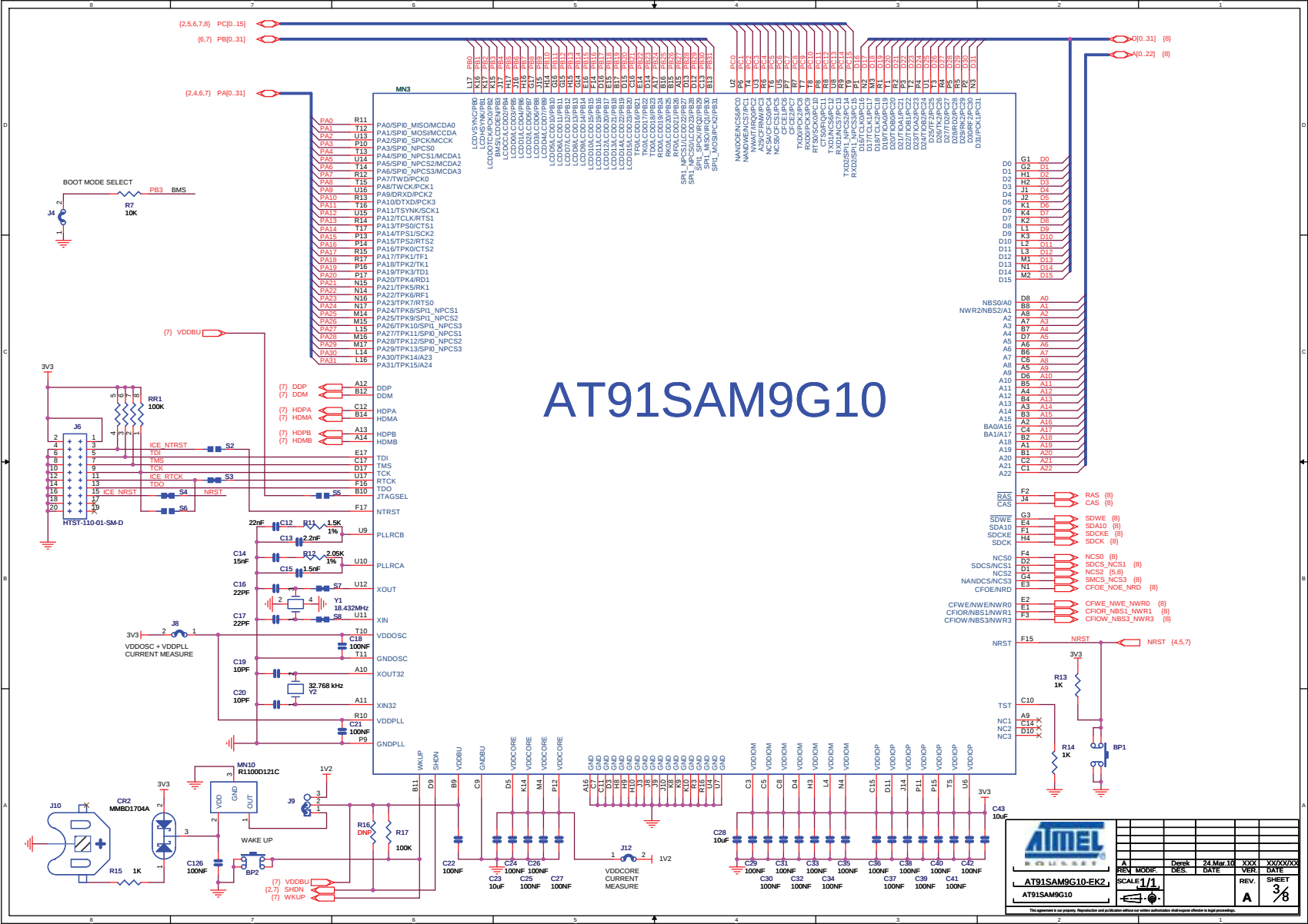
Figure 7-3. SAM9G10 Microcontroller
