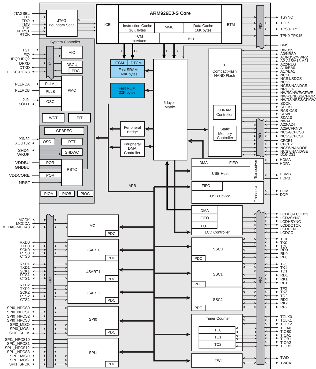
Figure 5-1. Block Diagram
