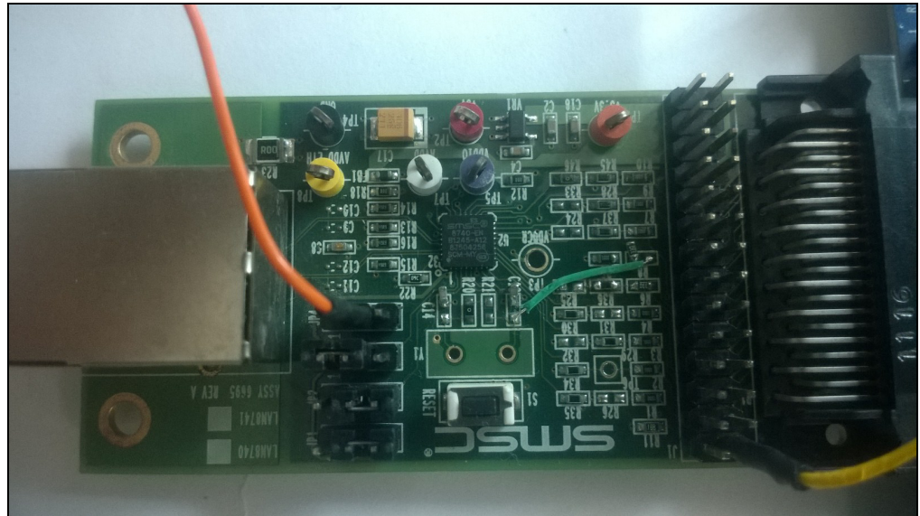
FIGURE 3-5: LAN8740
