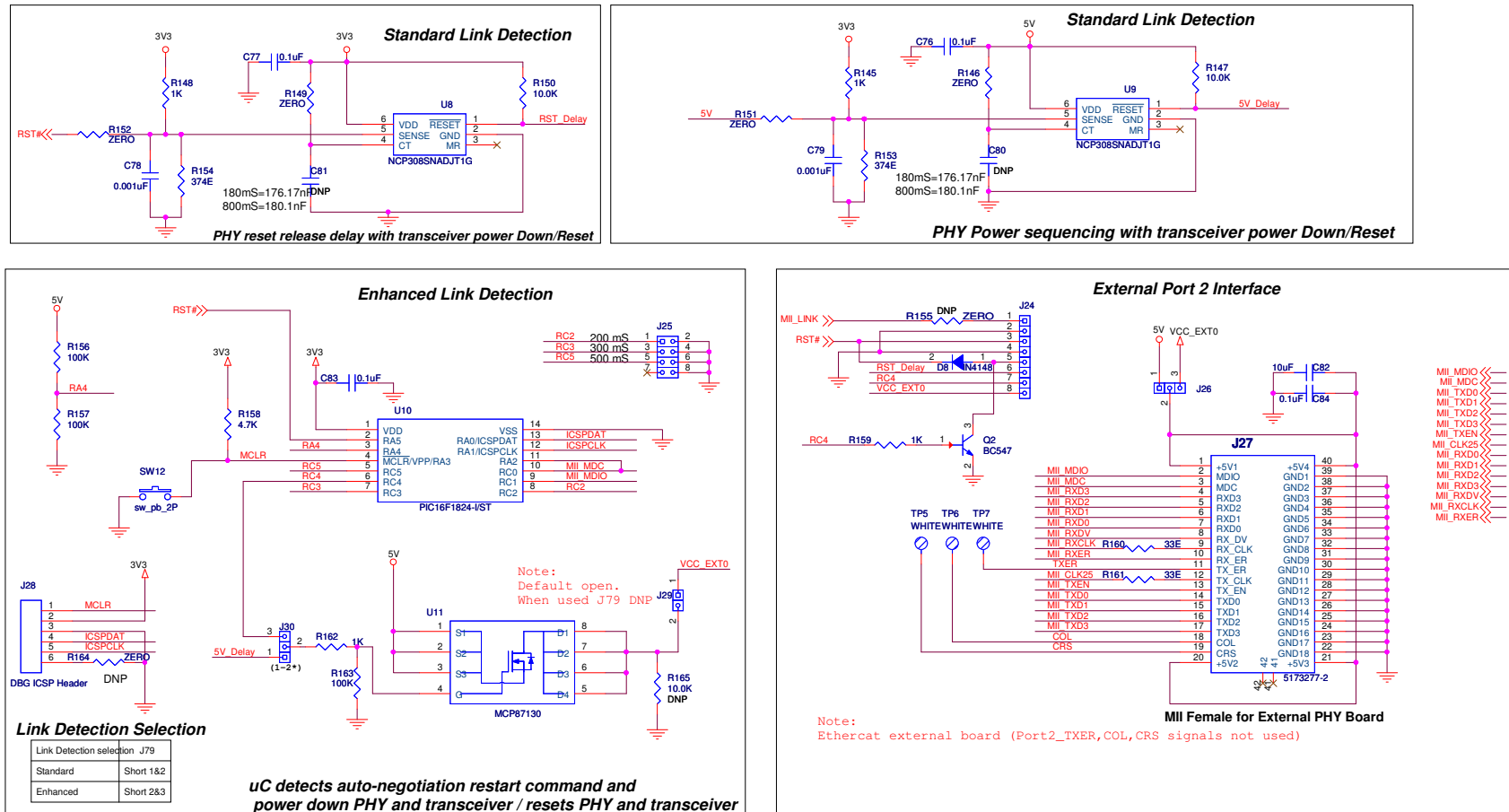
FIGURE B-10: ENHANCED LINK DETECTION
