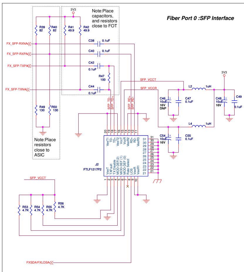
FIGURE B-5: SFP INTERFACE
