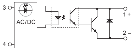
Figure 3 — DX relays
