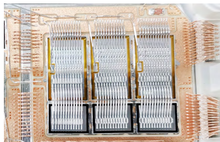
Figure 8: DBC/DBC, DBC/Power terminal wire bonding
