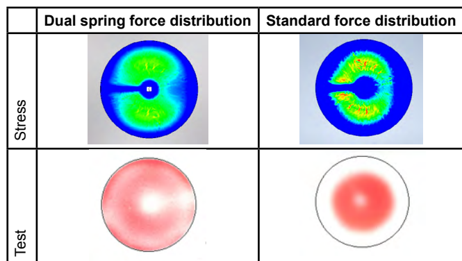
Figure 4: Comparison of standard force distribution with dual spring force distribution
