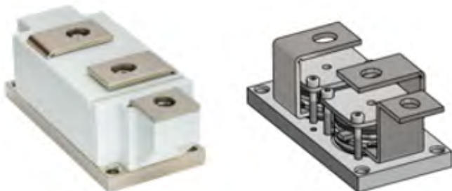
Figure 2: 60Pak BiPolar module
