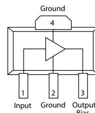
Functional Block Diagram (SOT-89)
