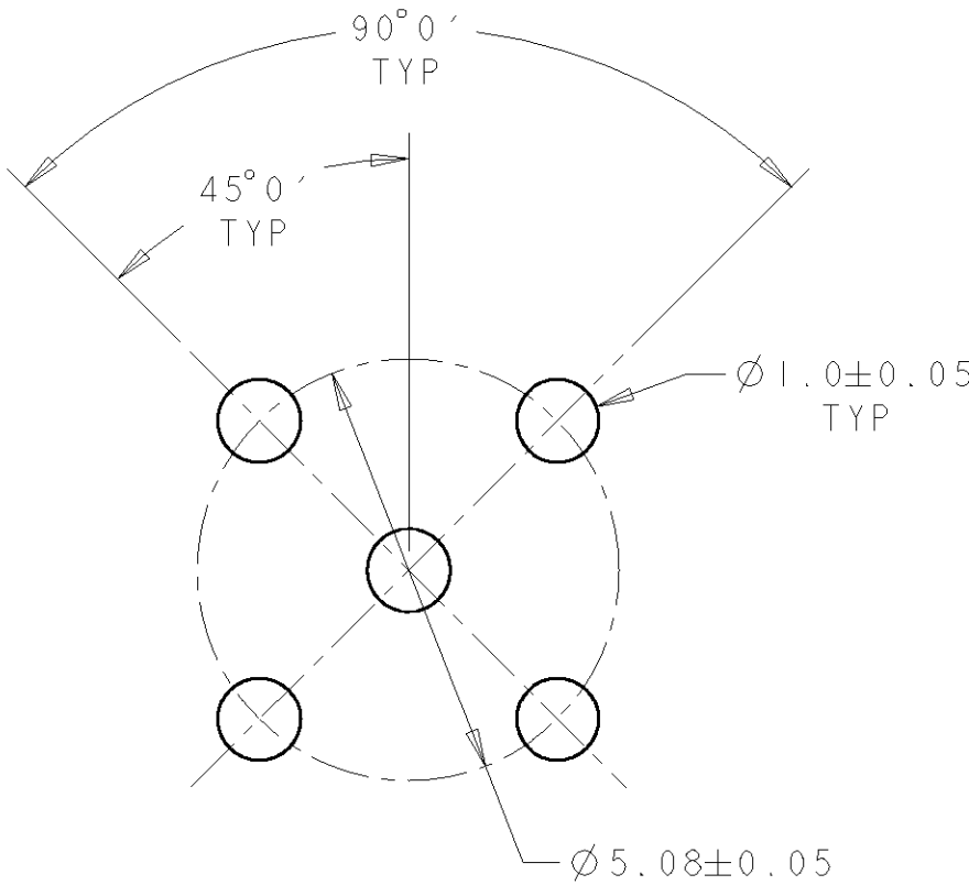
RECOMMENDED PC BOARD LAYOUT SCALE 10:1
