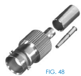
FIG. 48 RFB-1123-1, -1-SS, -C1, -C2, RFB-1124-1P, -1X
