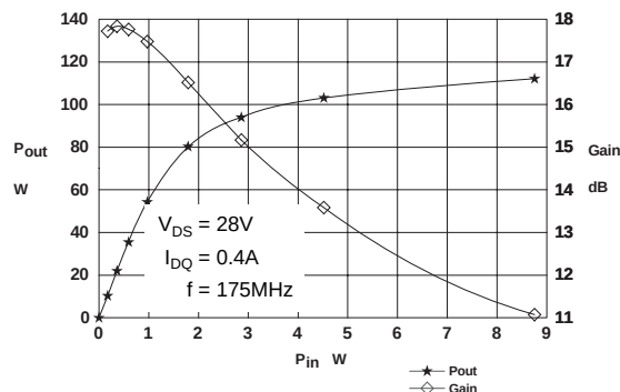
Figure 2 – Power Output & Gain vs. Power Input.
