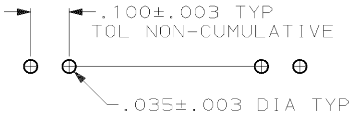
RECOMMENDED HOLE LAYOUT
