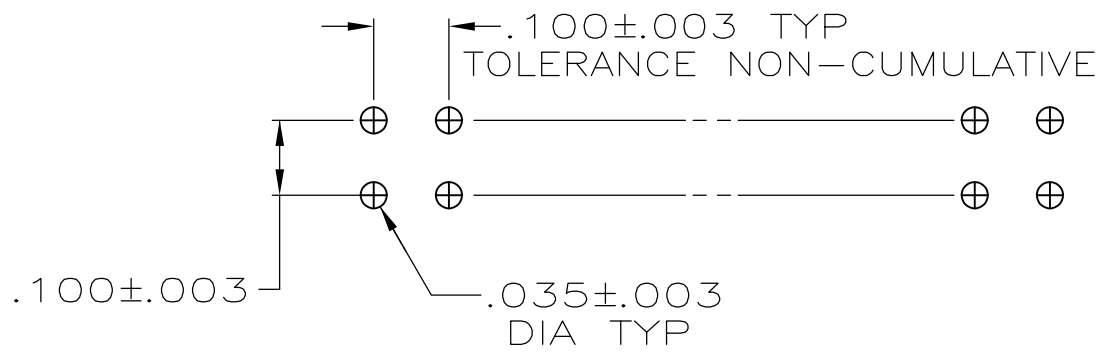
RECOMMENDED HOLE LAYOUT FOR MANUAL INSERTION
