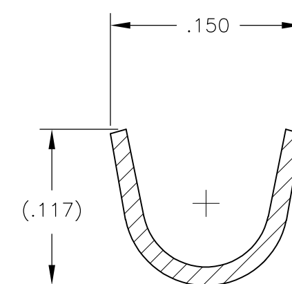
SECTION X-X
