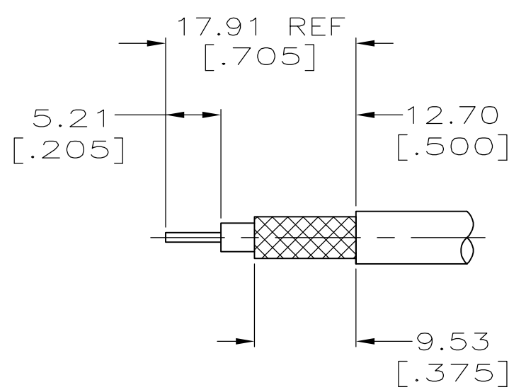
VIEW X RECOMMENDED STRIP LENGTH
