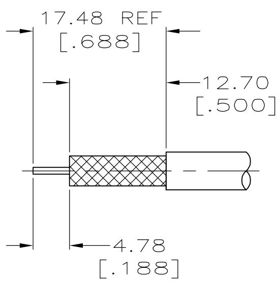
VIEW W RECOMMENDED STRIP LENGTH
