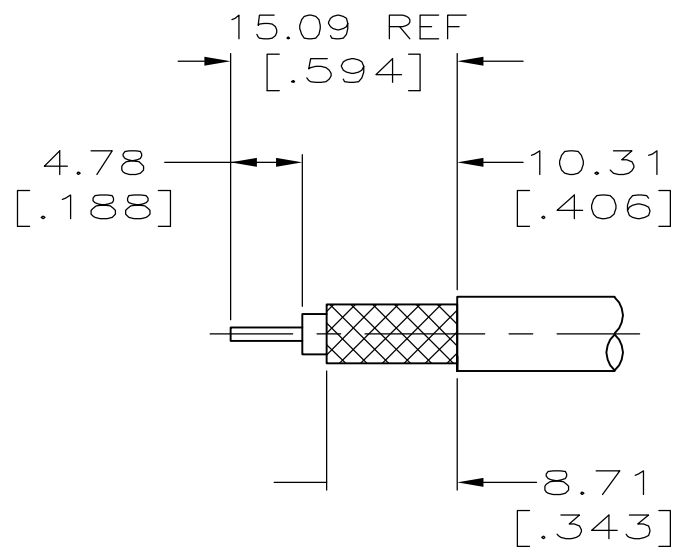
VIEW U RECOMMENDED STRIP LENGTH
