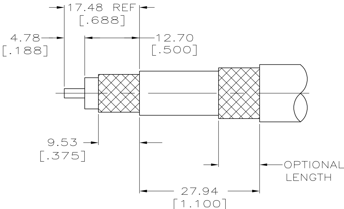
VIEW A RECOMMENDED STRIP LENGTH SCALE 2:1 VIEW B
