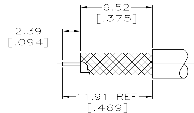
RECOMMENDED STRIP LENGTH SCALE 4:1
