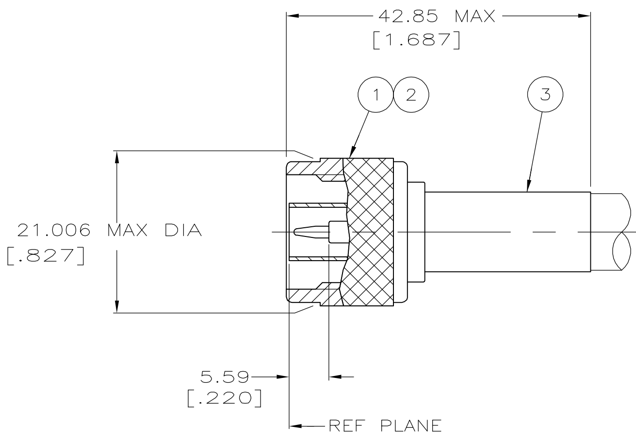
VIEW X
