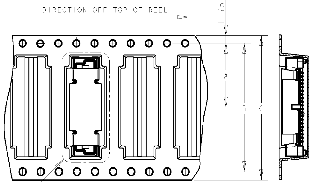
DETAIL B
