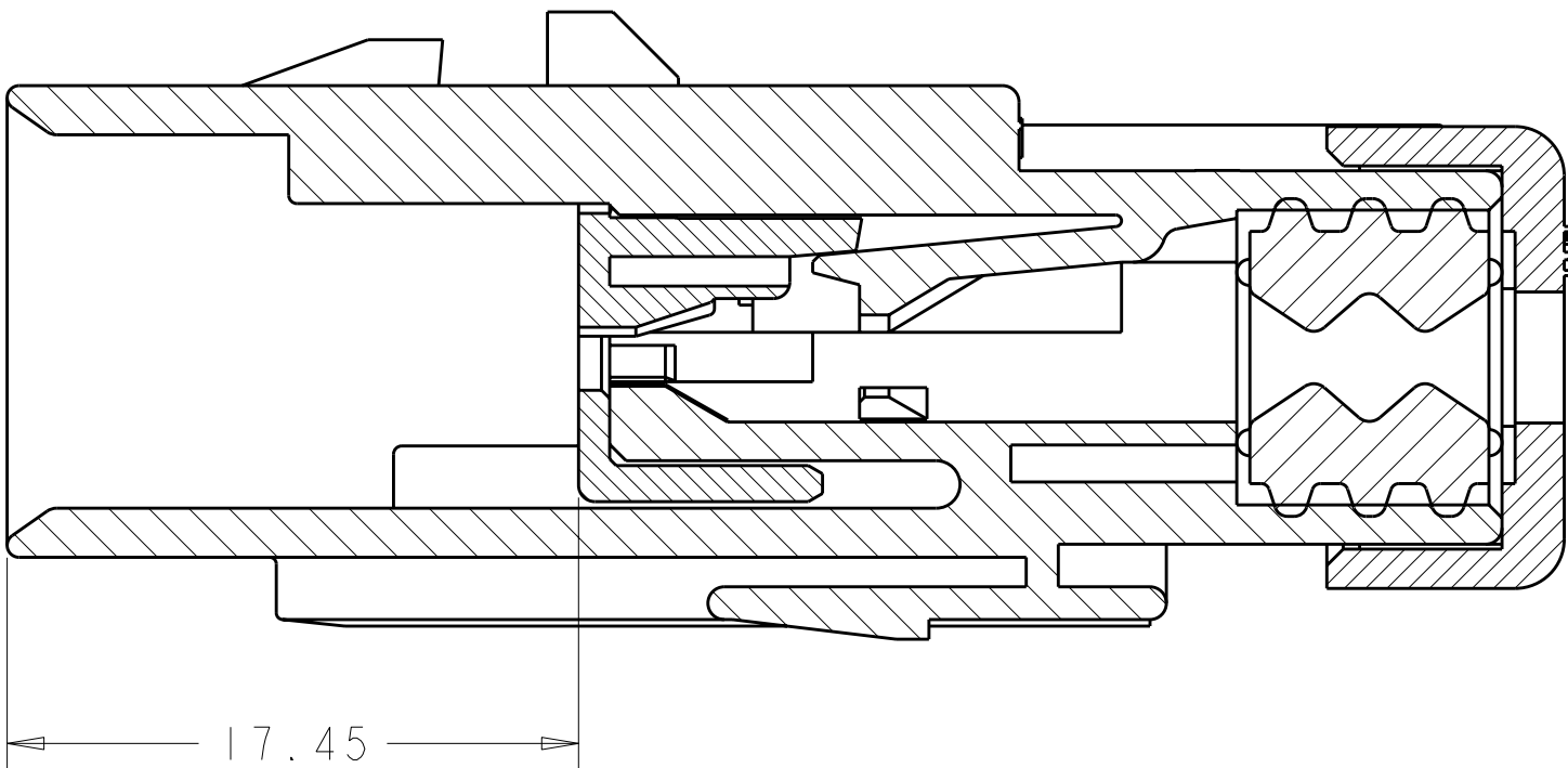
SECTION A - A WITH TPA IN CLOSED POSITION
