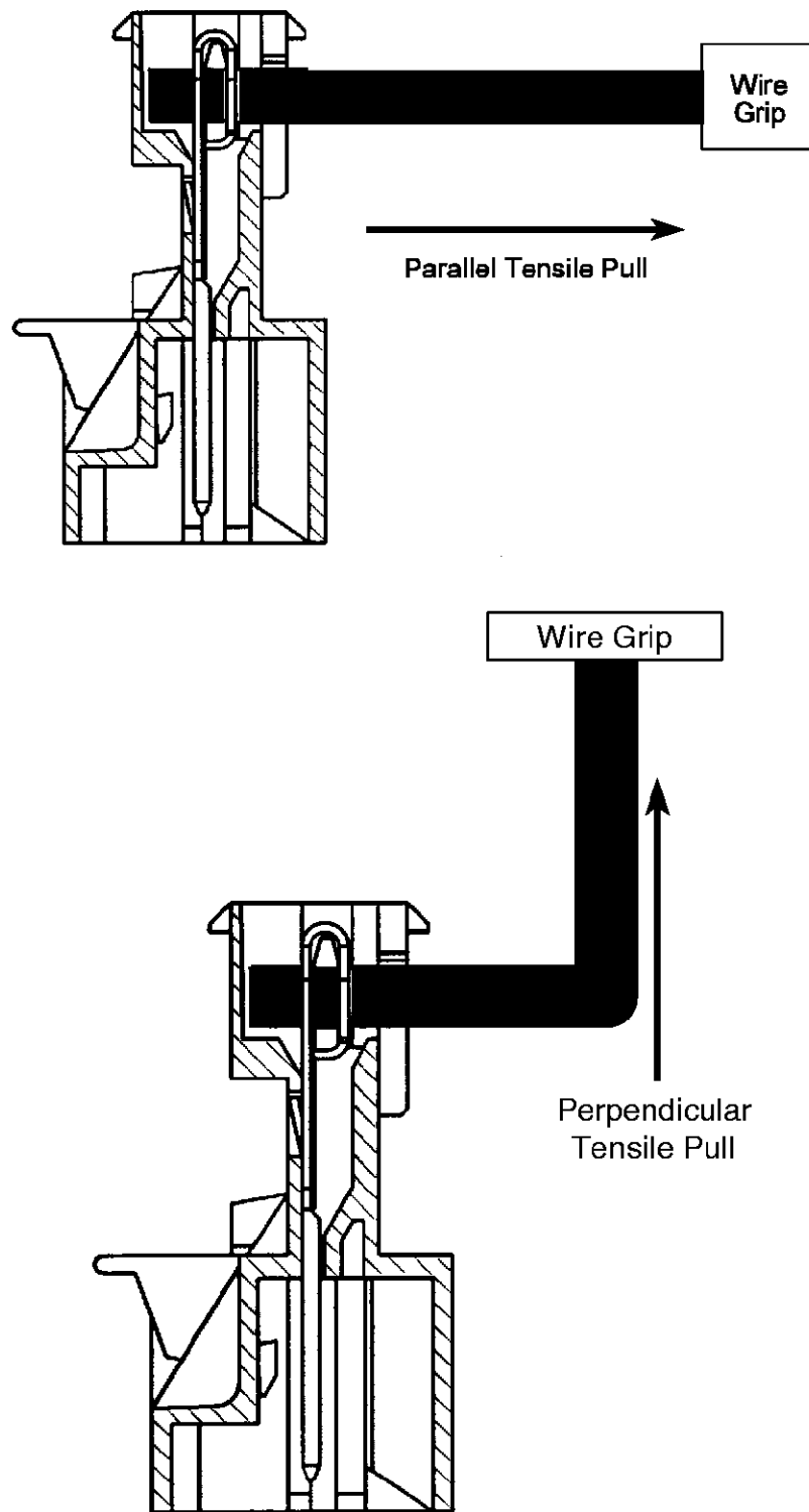
Figure 5 Termination Tensile Strength
