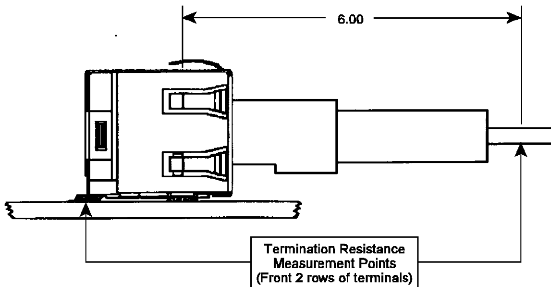
Figure 3 Dry Circuit Resistance Measurement Points
